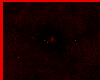
Omega Centauri. Credit: NASA/JPL-Caltech/WISE Team
