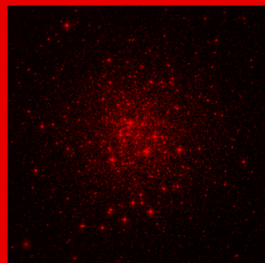
M72: A Globular Cluster of Stars. Credit: NASA, ESA, Hubble, HPOW
