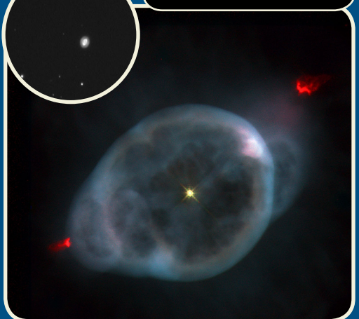
Ghost of Jupiter as seen by Hubble - HST/NASA/ESA
