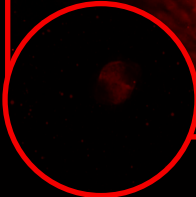
Dumbbell Nebula as seen by the Very Large Telescope (ESO)
