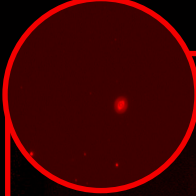
Ghost of Jupiter as seen by Hubble - HST/NASA/ESA
