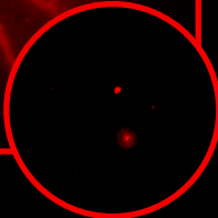
Lion Nebula as seen by Hubble - NASA/Andrew Fruchter (STScI)
